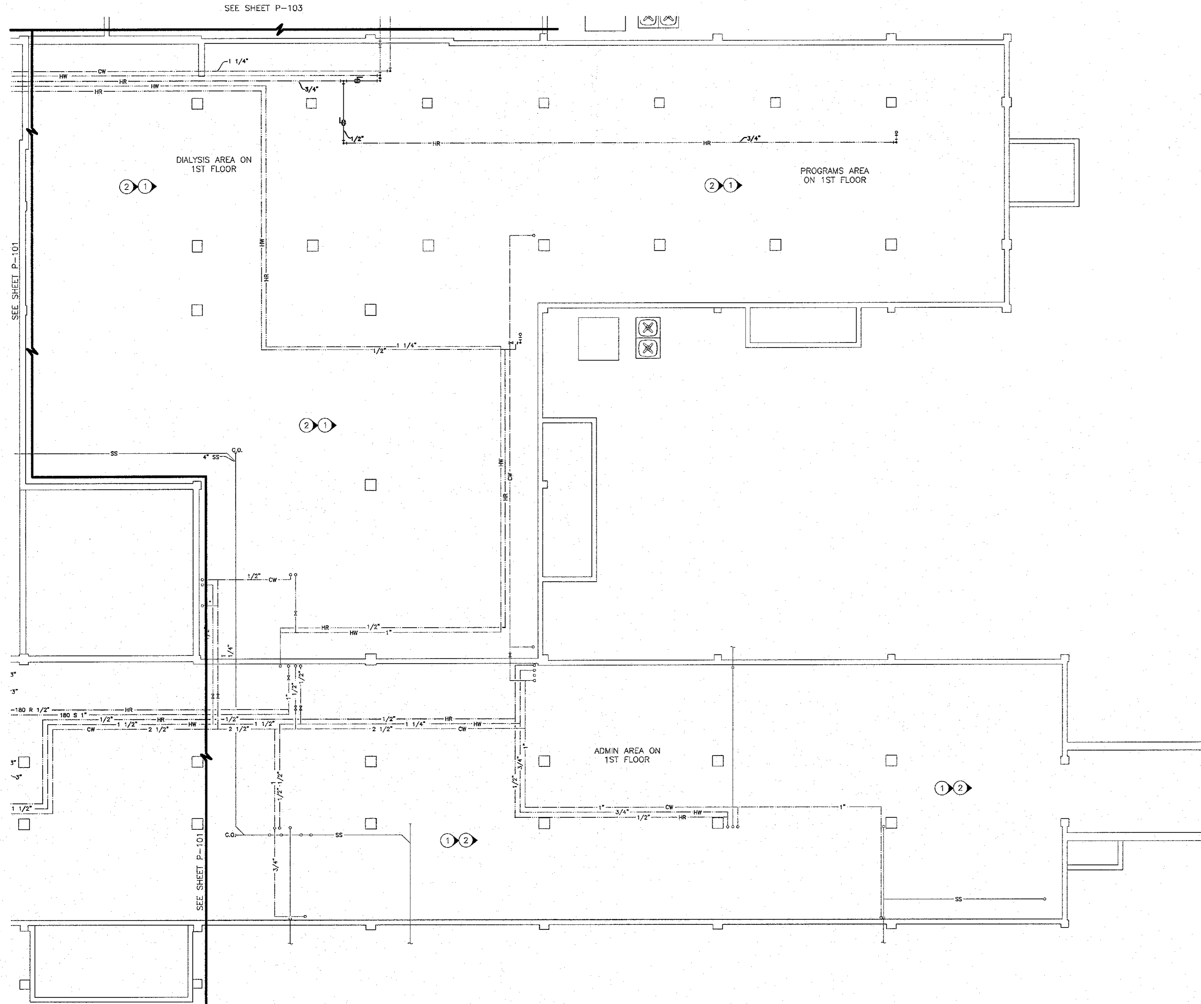
① PARTIAL CRAWL SPACE PIPING DEMOLITION AND RENOVATION PLAN SCALE: 1/8"=1'-0"
