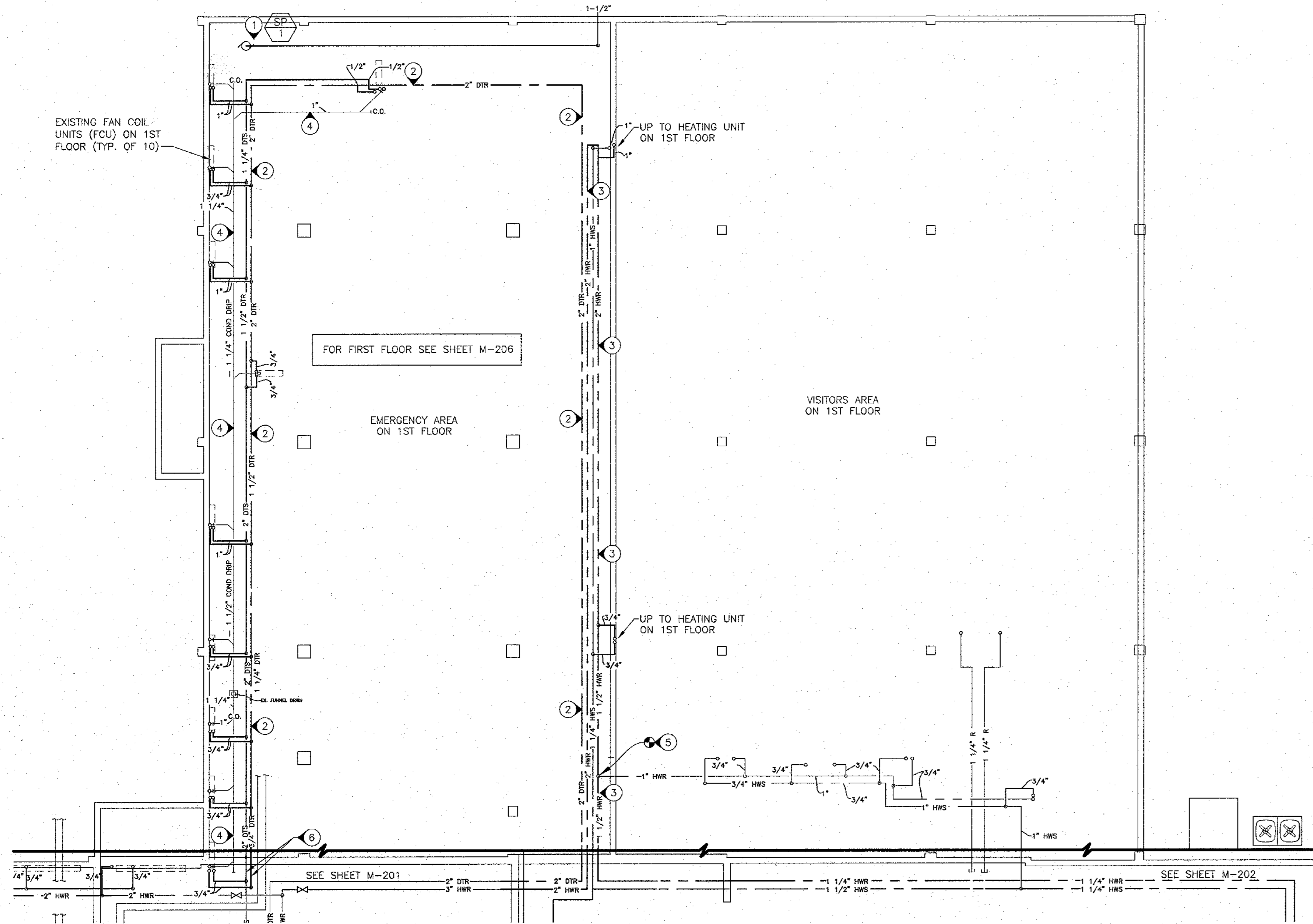
① PARTIAL CRAWL SPACE HVAC PIPING RENOVATION PLAN SCALE: 1/8"=1'-0"
