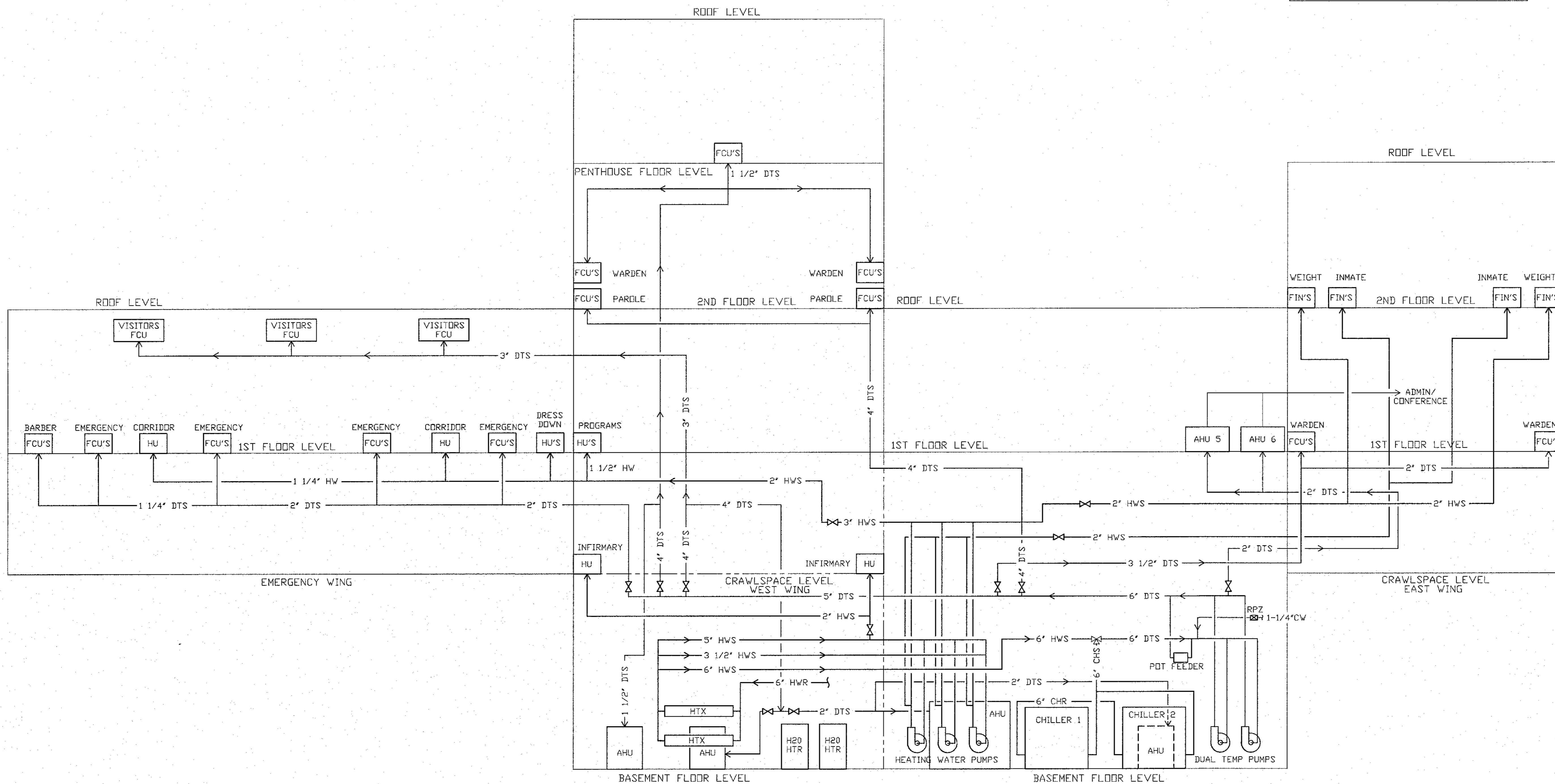
1 ADMINISTRATION BUILDING HYDRONIC RISER DIAGRAM (VIEW WEST) SCALE: NONE
