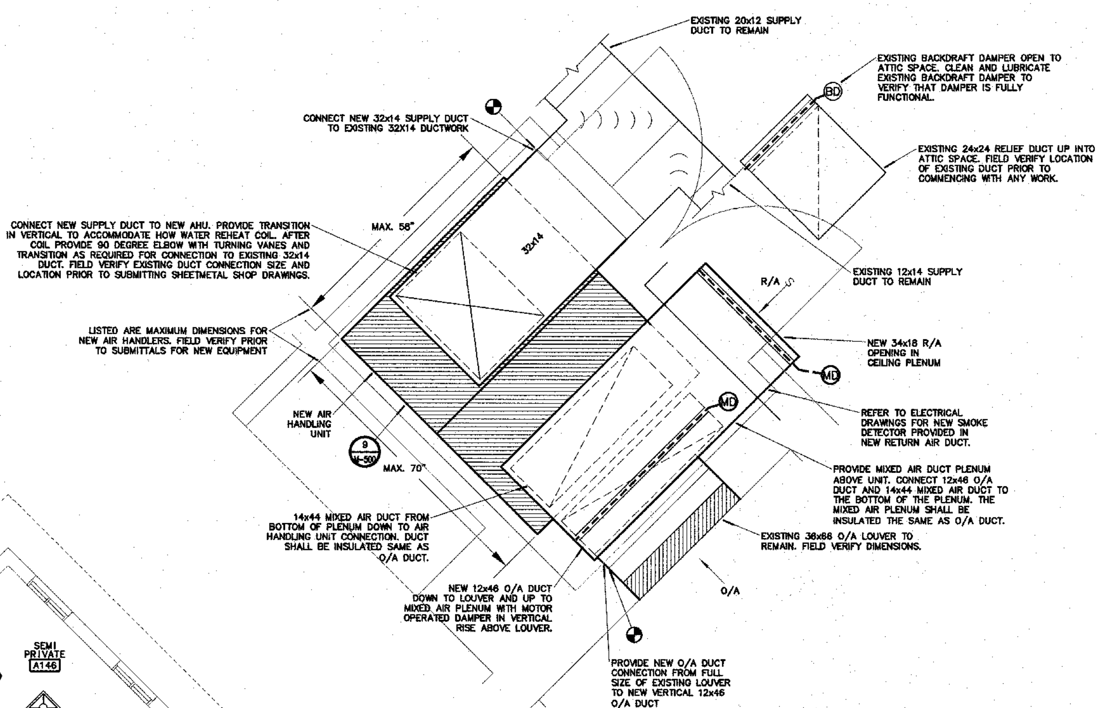
2 TYPICAL WING *AHU5 THRU 10* ENLARGED FLOOR PLAN M-106 SCALE: 1/2"=1'-0"
