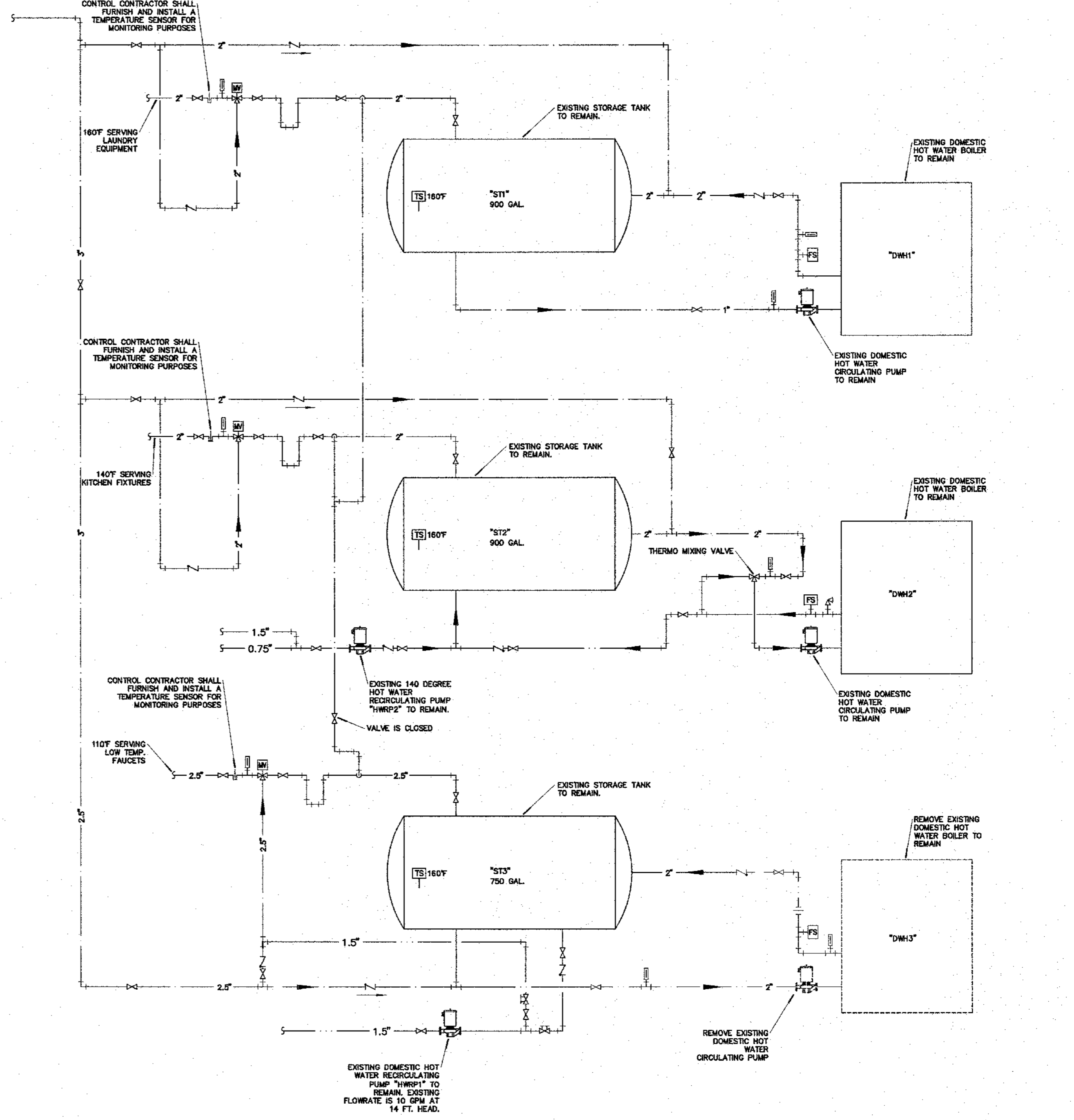
1 DOMESTIC HOT WATER FLOW DIAGRAM - DEMOLITION M-602 NO SCALE
