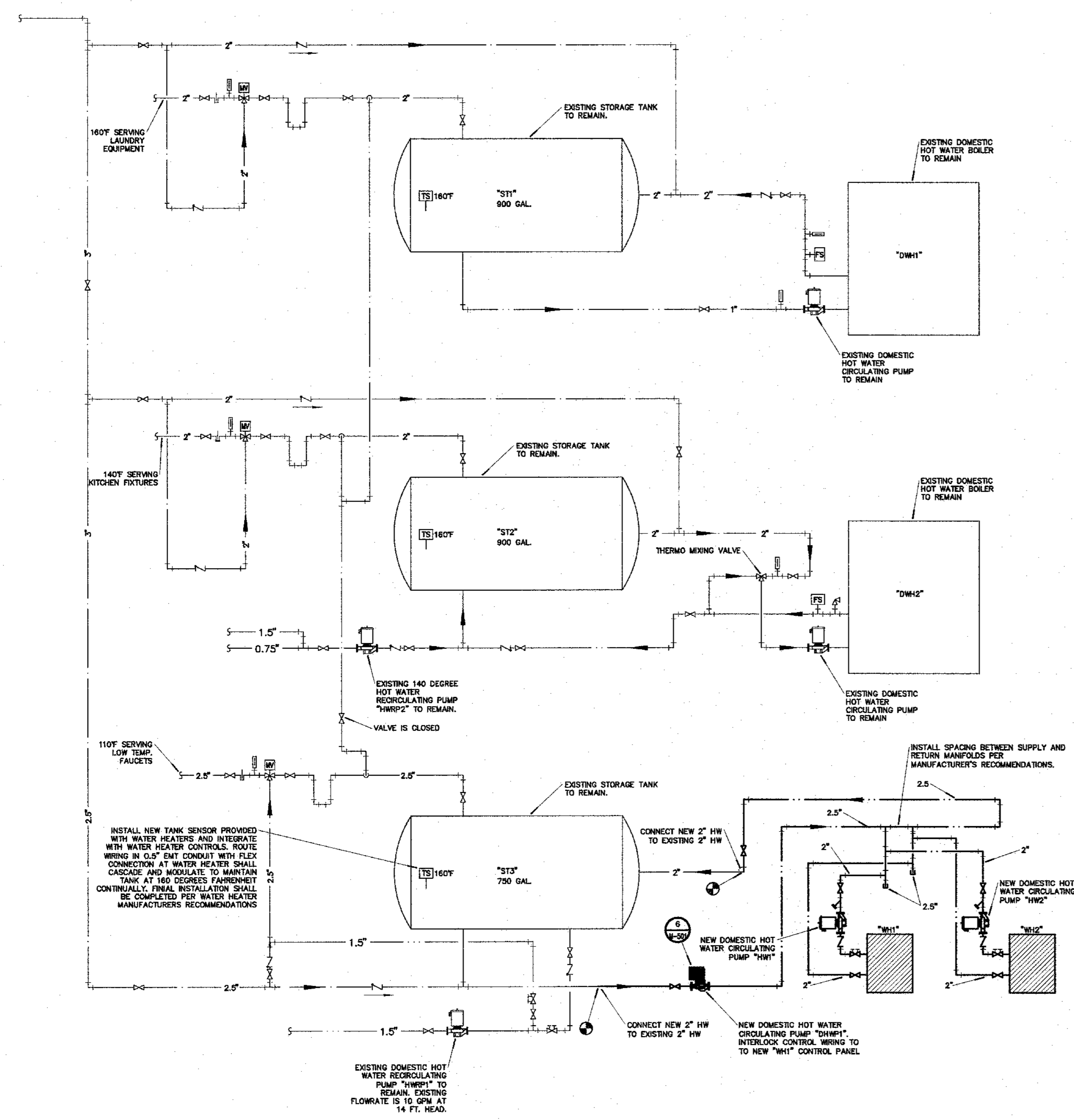
2 DOMESTIC HOT WATER FLOW DIAGRAM - IMPROVEMENT M-602 NO SCALE
