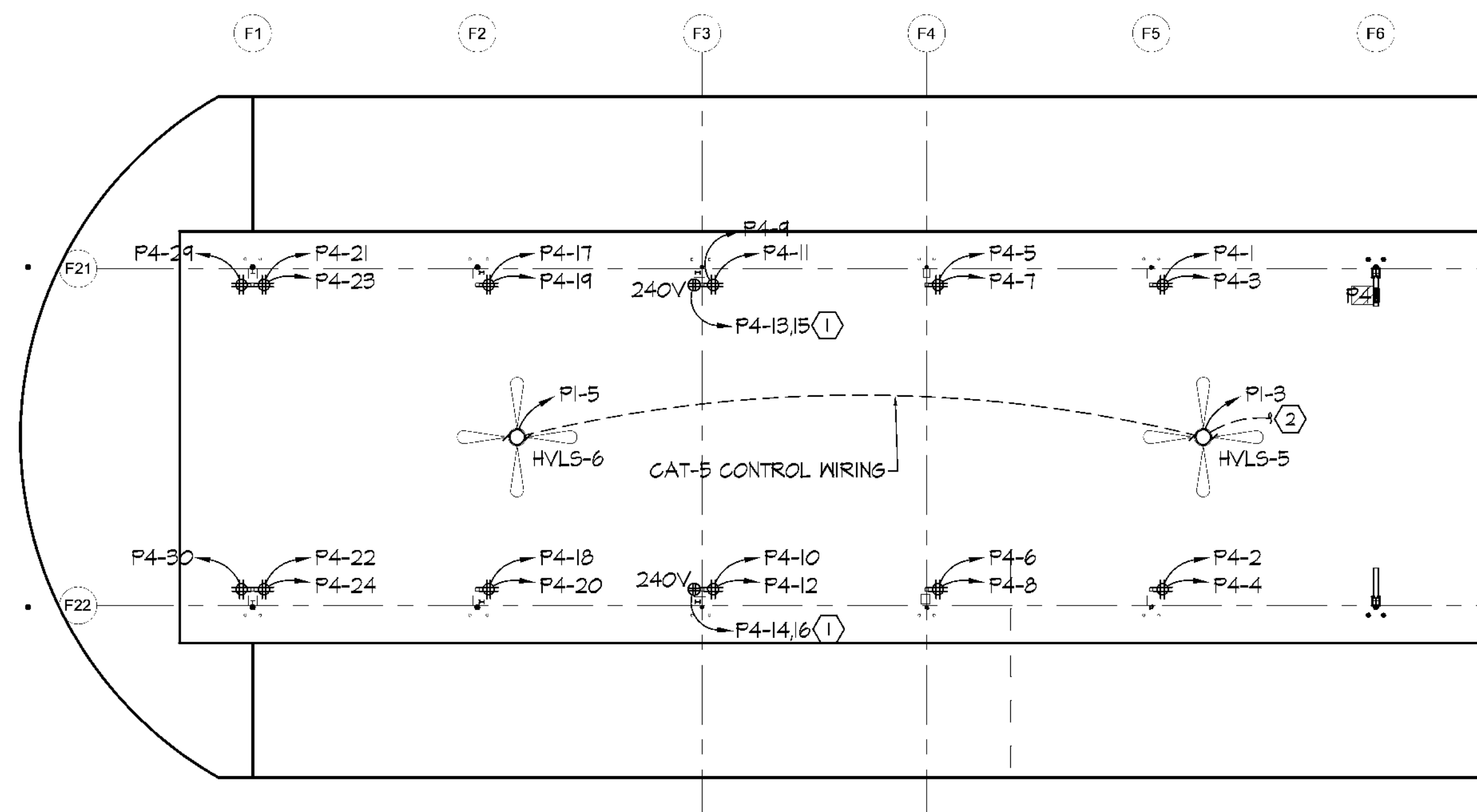
02 FMB WEST POWER FLOOR PLAN SCALE: 1/16"=1'-0"
