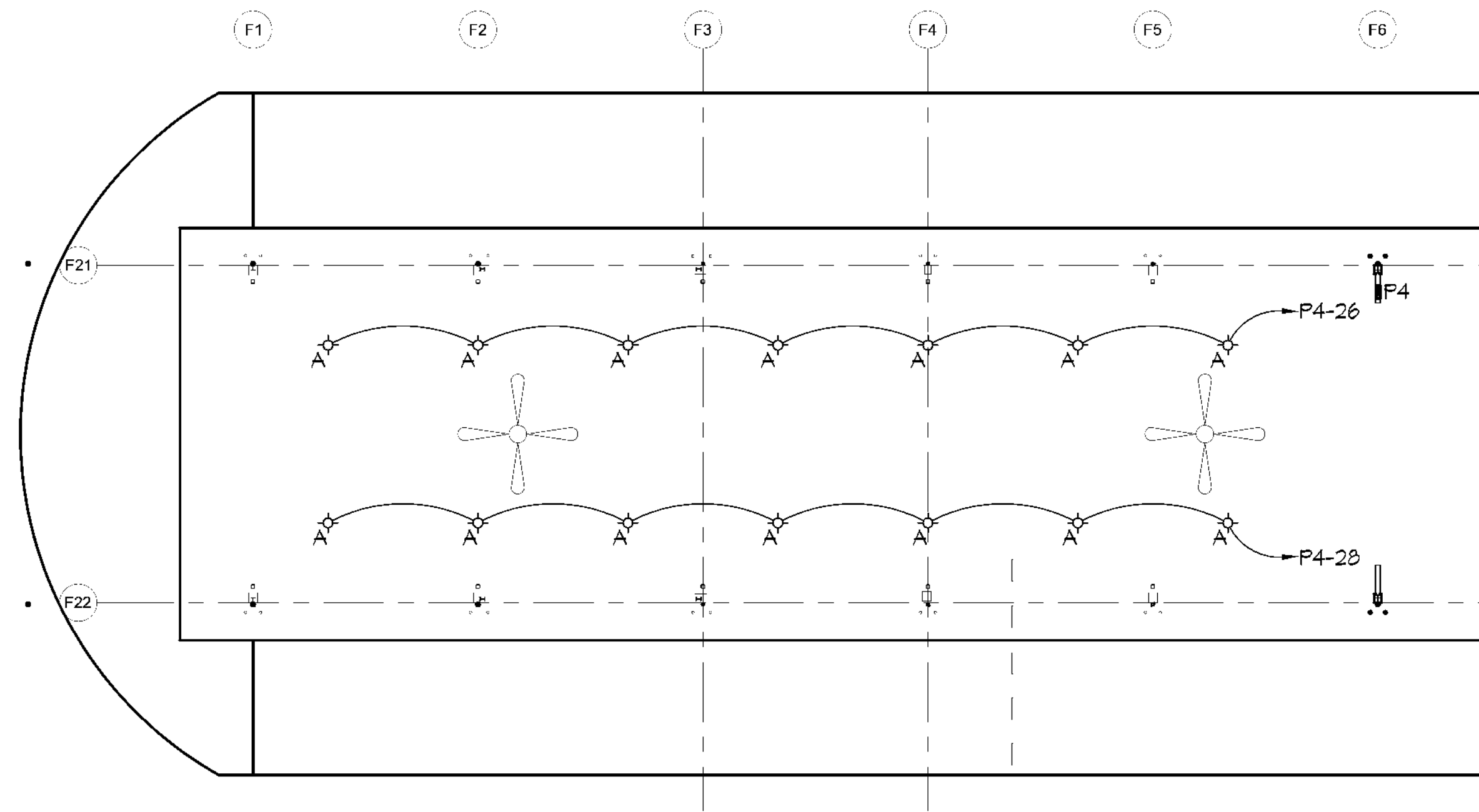
01 FMB WEST LIGHTING FLOOR PLAN SCALE: 1/16"=1'-0"
