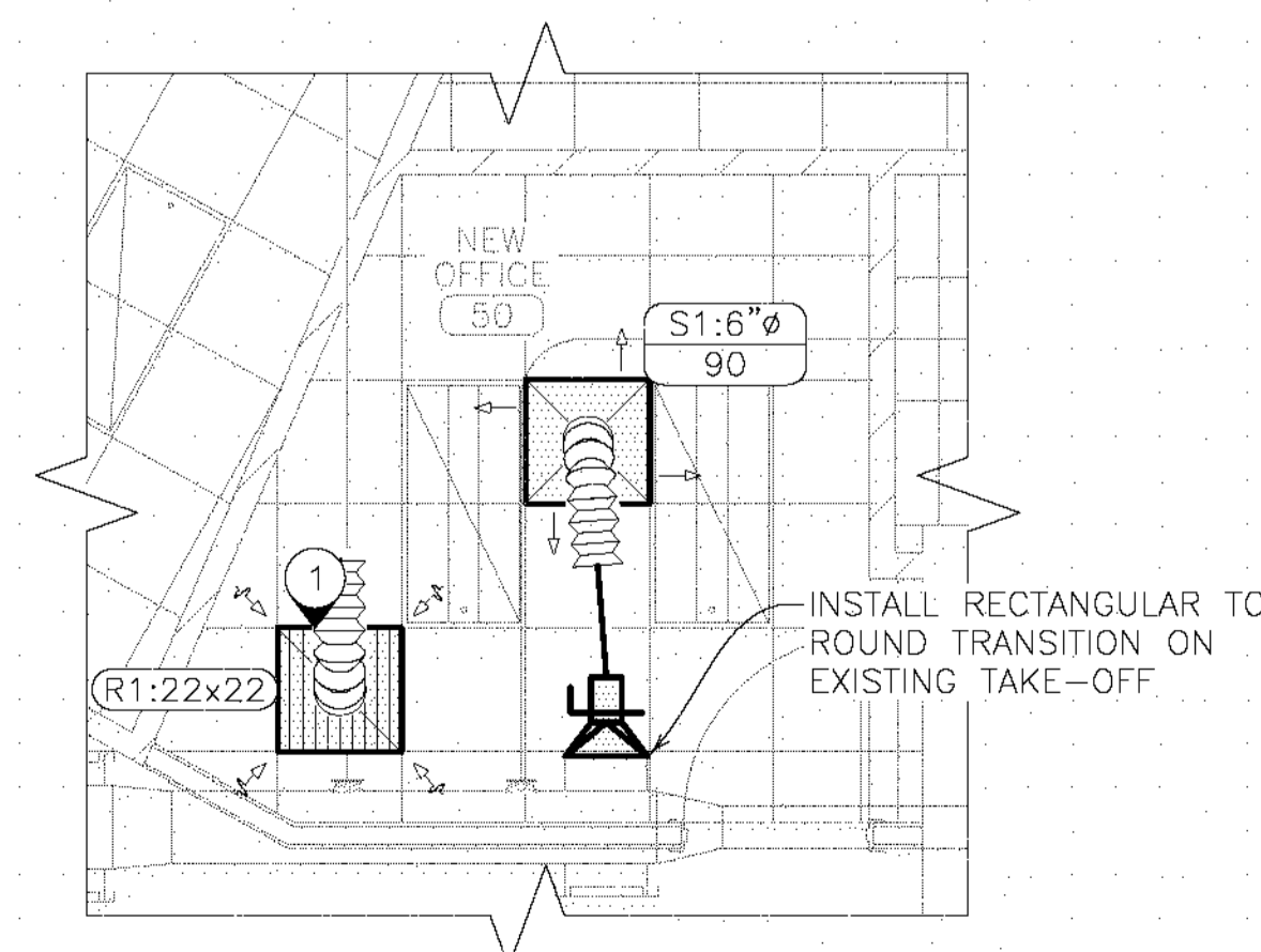
3 NEW CENTRAL OFFICE - MECHANICAL HVAC PLAN SCALE: 1/4"=1'-0"
