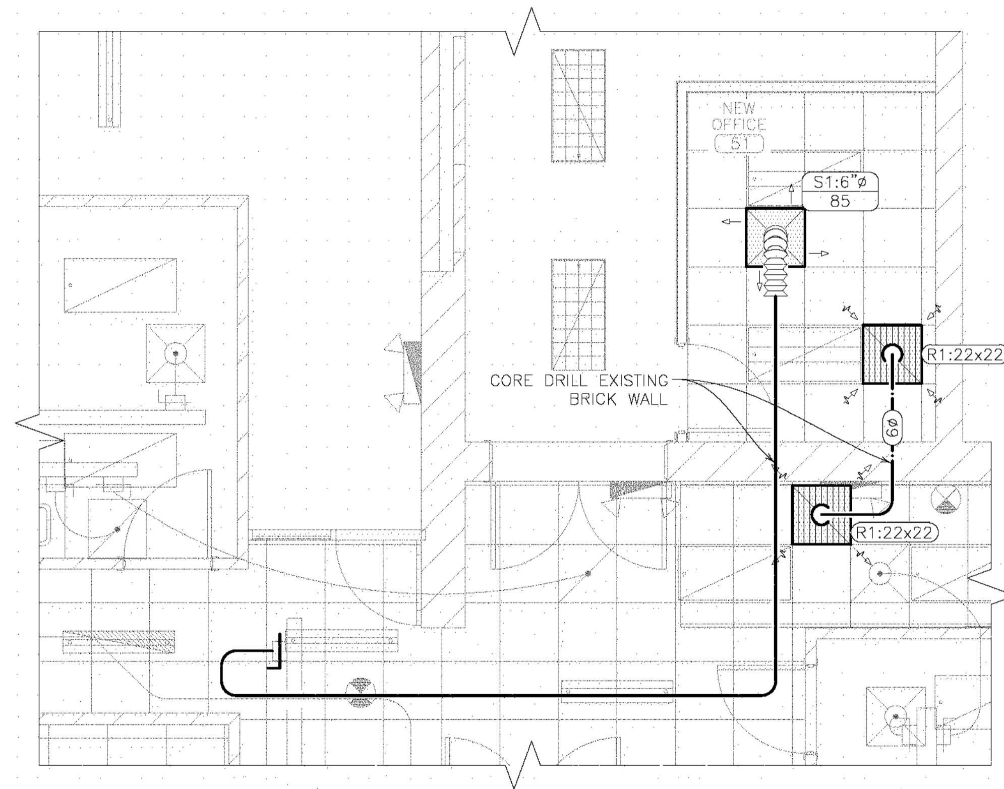
2 NEW OFFICE - MECHANICAL HVAC PLAN SCALE: 1/4"=1'-0"
