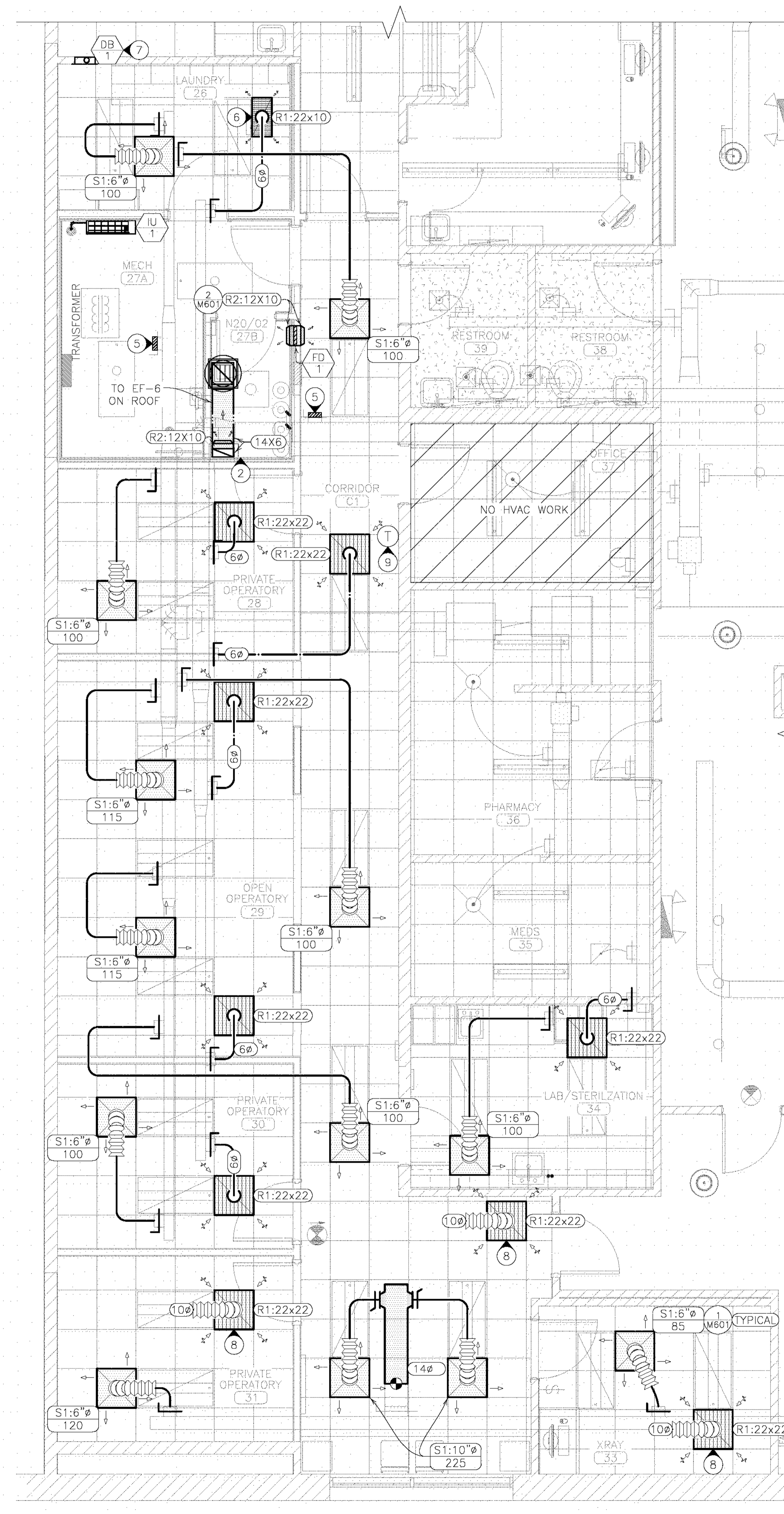
4 DENTAL CLINIC - MECHANICAL HVAC PLAN SCALE: 1/4"=1'-0"
