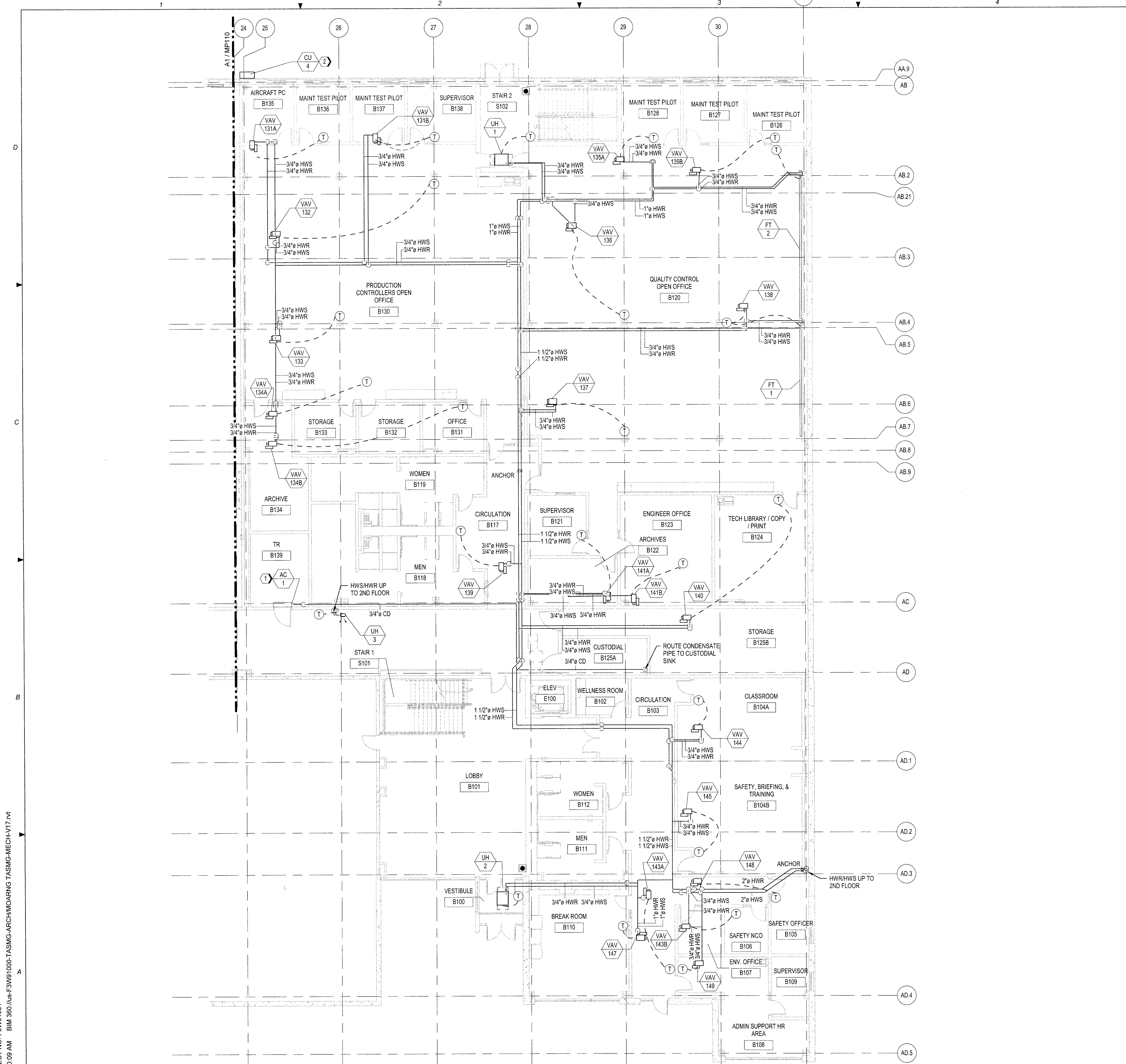
A1 PARTIAL FIRST FLOOR PIPING PLAN - AREA A 1/8" = 1'-0"
