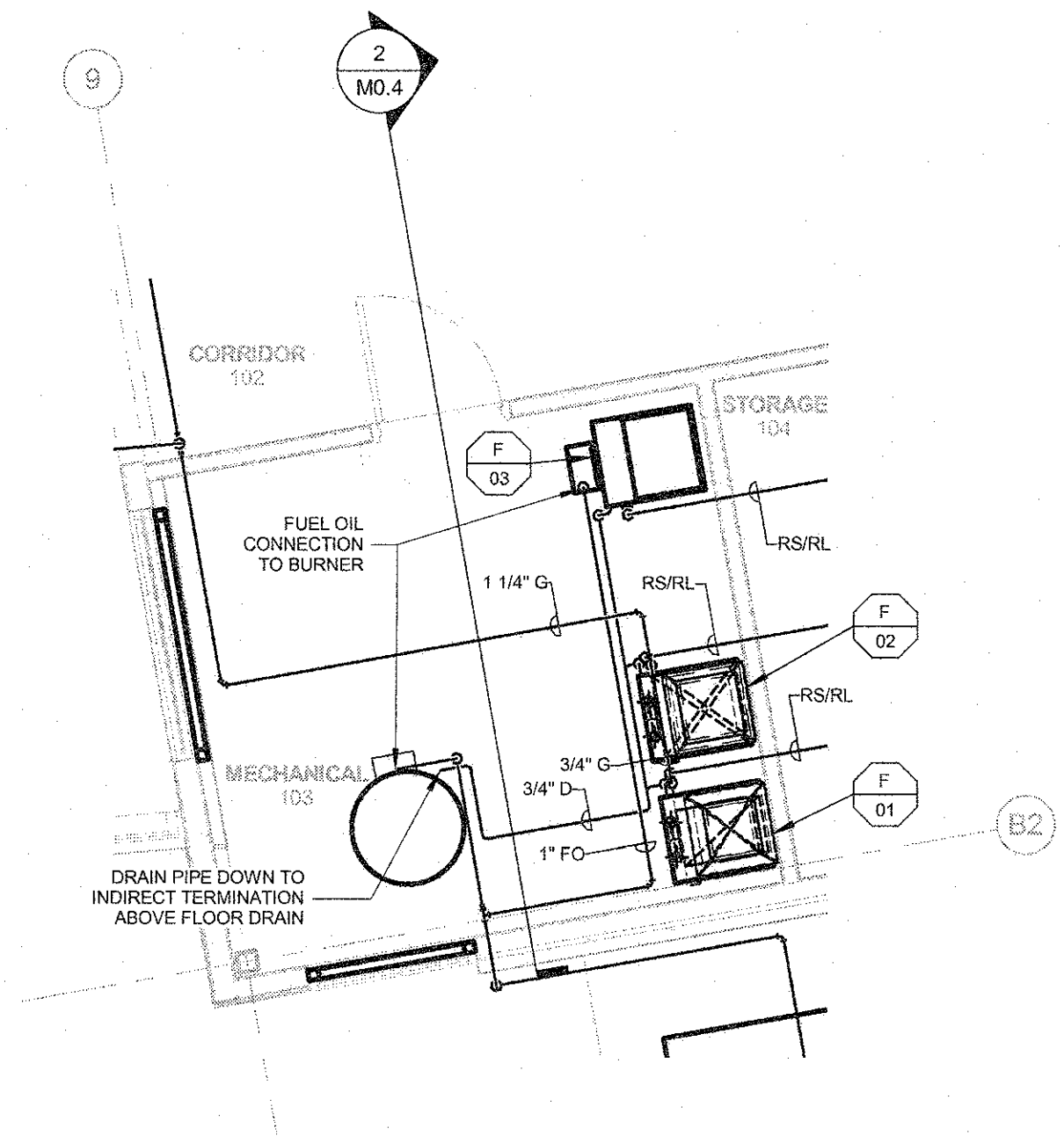
4 ENLARGED MECHANICAL PIPING PLAN SCALE: 1/4" = 1'-0"
