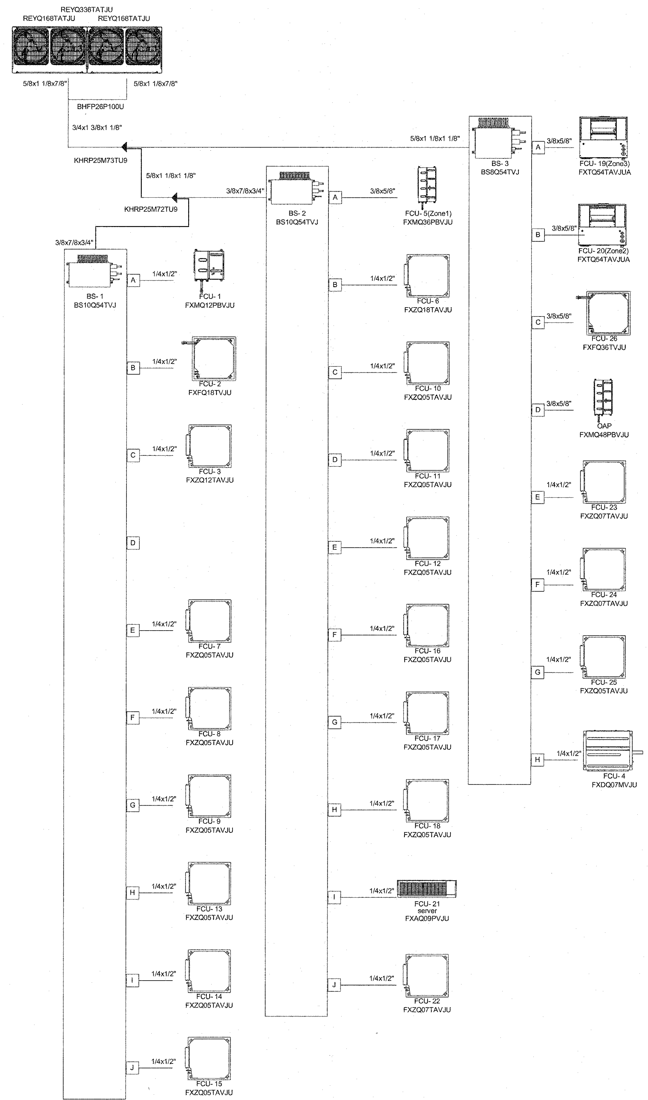
VRF Riser Diagram NOT TO SCALE
