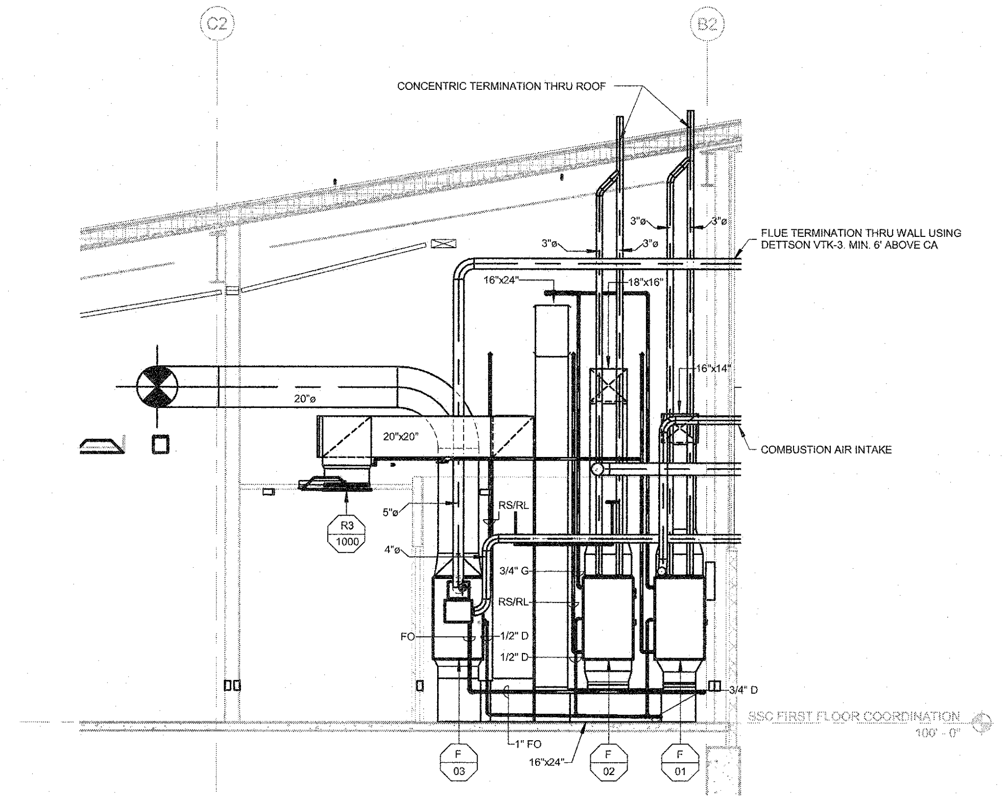
2 SECTION MECHANICAL 103 SCALE: 1/4" = 1'-0"
