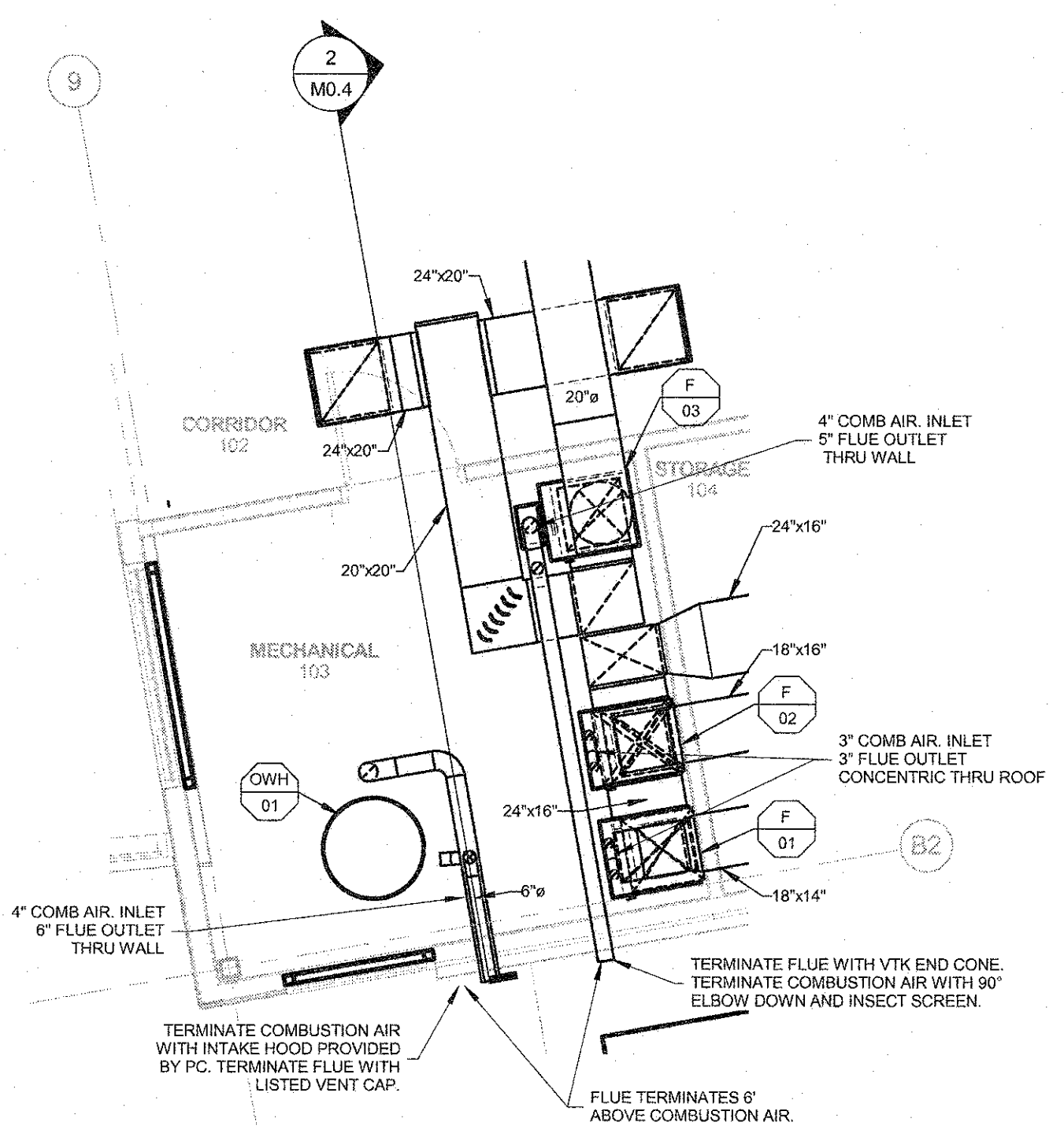
3 ENLARGED MECHANICAL DUCTWORK PLAN SCALE: 1/4" = 1'-0"
